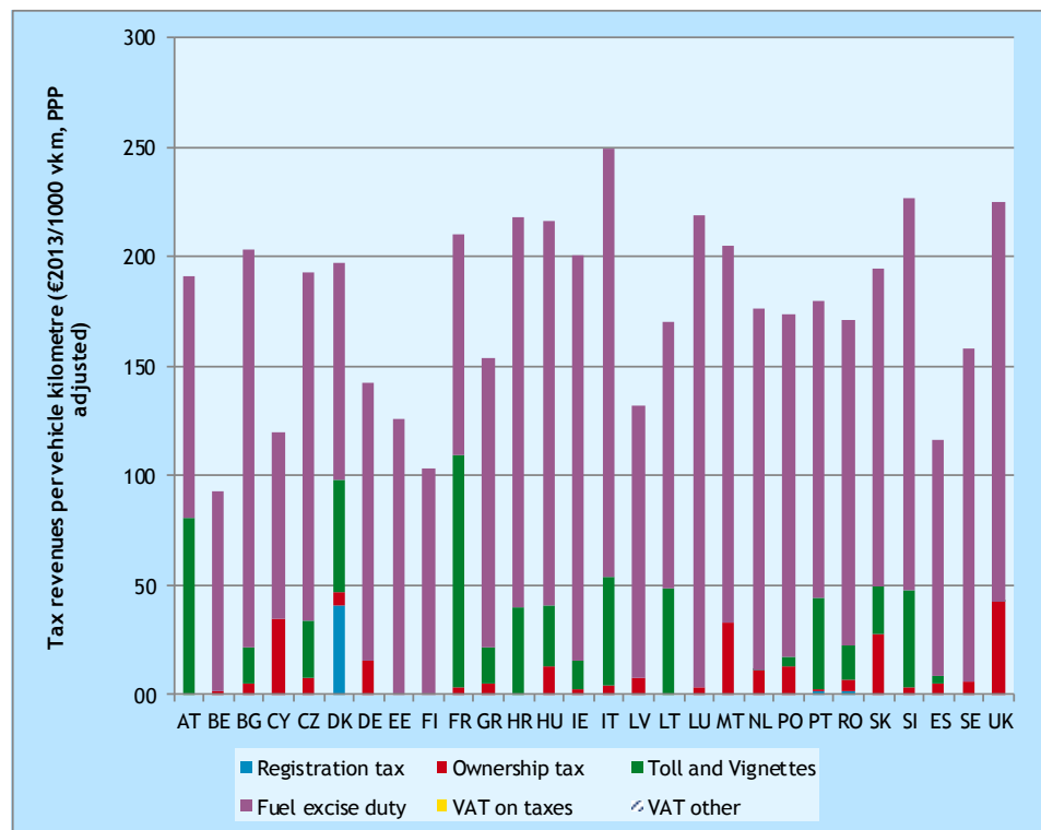
Figure 51 Average revenue from taxes and charges for busses in 2013
