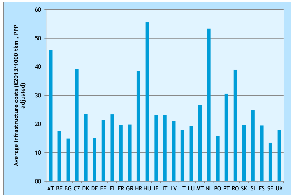
Figure 39 Average infrastructure costs HGVs in 2013
