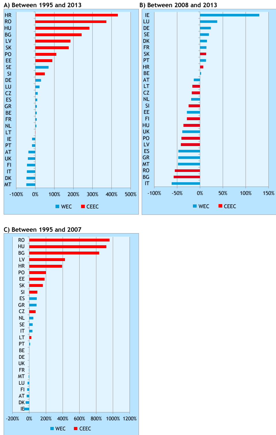
Figure 24 Change in O&M expenditures over time
